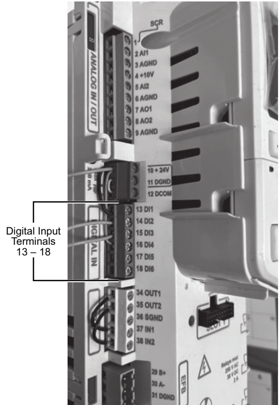
Fig. 59 — Digital Input Terminal Block Location on ACH580 VFD
