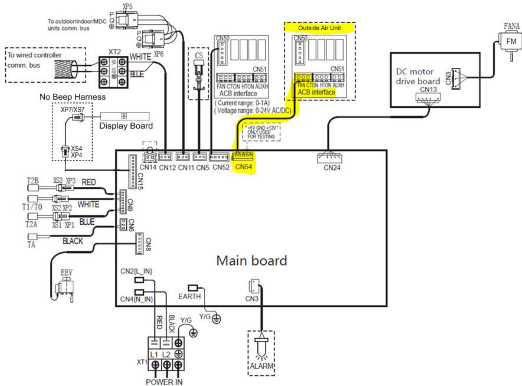
Fig. 15 —40VMZ09-024 Typical Wiring Diagram
